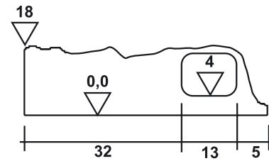
Spant F / 50 x 18 cm
